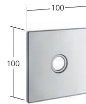
Escutcheon for sliding wall bar
